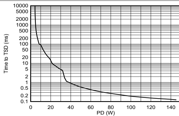
图 7-28. Time to Thermal Shut-Down During Inrush State
