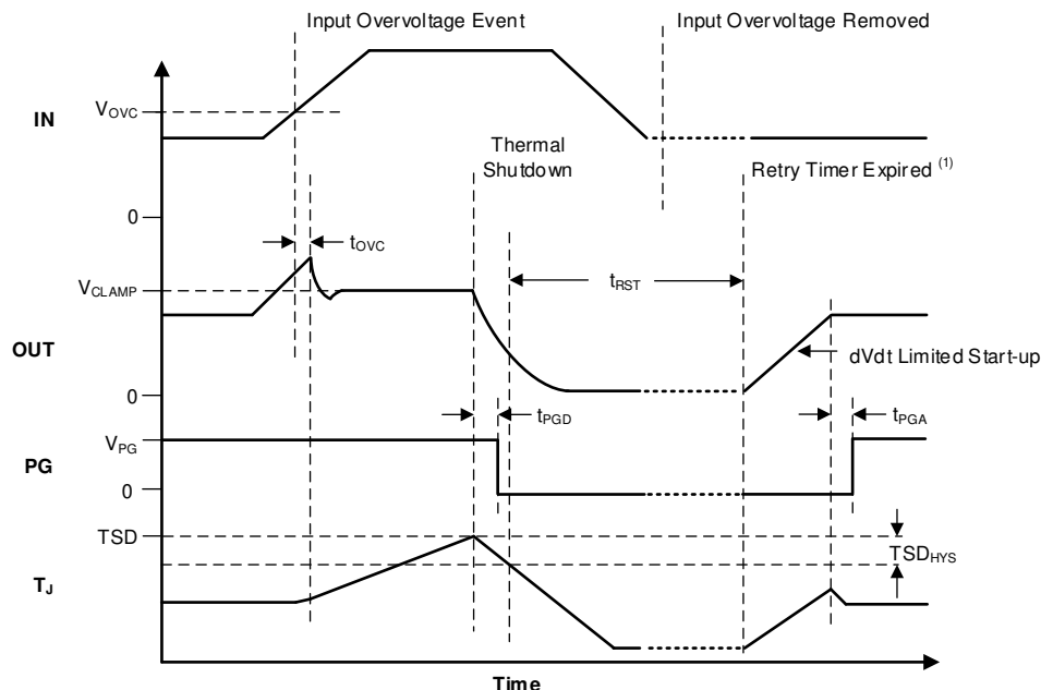
图 8-8. TPS25972x Overvoltage Response (Auto-Retry)
