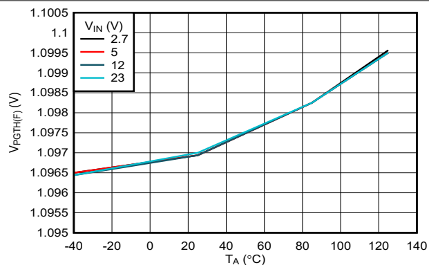
图 7-26. PGTH Threshold (Falling) vs Temperature (TPS25972x, TPS25974x Variants)
