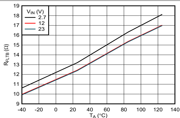
图 7-27. FLT Pin Pulldown Resistance vs Temperature
