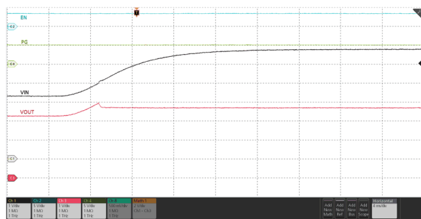
图 7-37. Overvoltage Clamp Response – TPS25972x
