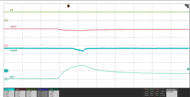
图 7-40. Active Current Limit Response – TPS25970x
