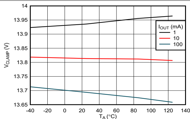
图 7-17. OVC Clamping Voltage (OVCSEL = 390 kΩ to GND) vs Load Current (TPS25972x Variant)
