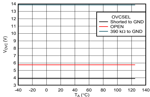
图 7-16. OVC Threshold vs Temperature (TPS25972x Variant)
