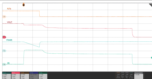
图 7-39. Overvoltage Clamp Response – TPS25972x
