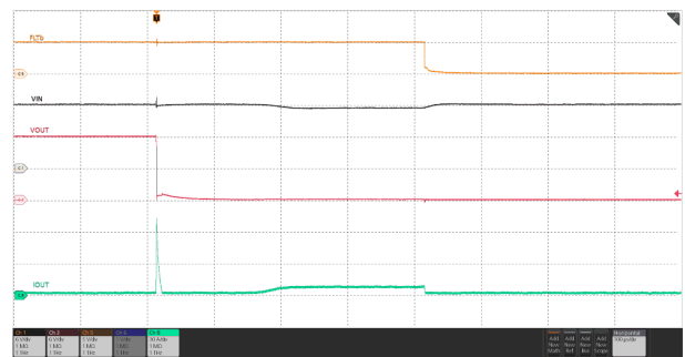
图 7-44. Output Short-Circuit During Steady State
