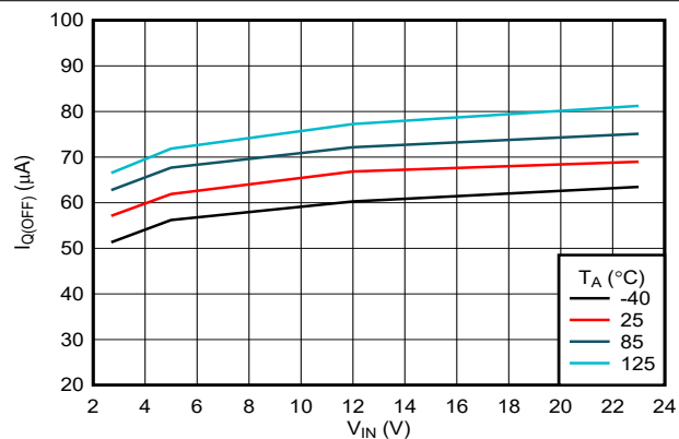
图 7-4. IN OFF State (UVLO) Current vs Temperature
