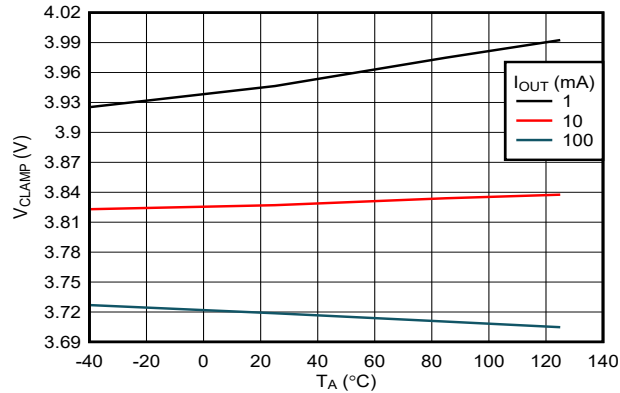
图 7-19. OVC Clamping Voltage (OVCSEL = GND) vs Load Current (TPS25972x Variant)
