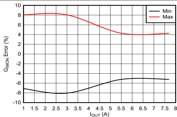
图 7-14. Analog Current Monitor Gain Accuracy
