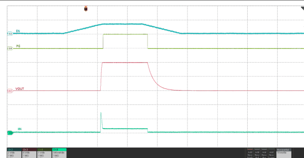
图 7-28. Time to Thermal Shut-Down During Inrush State
