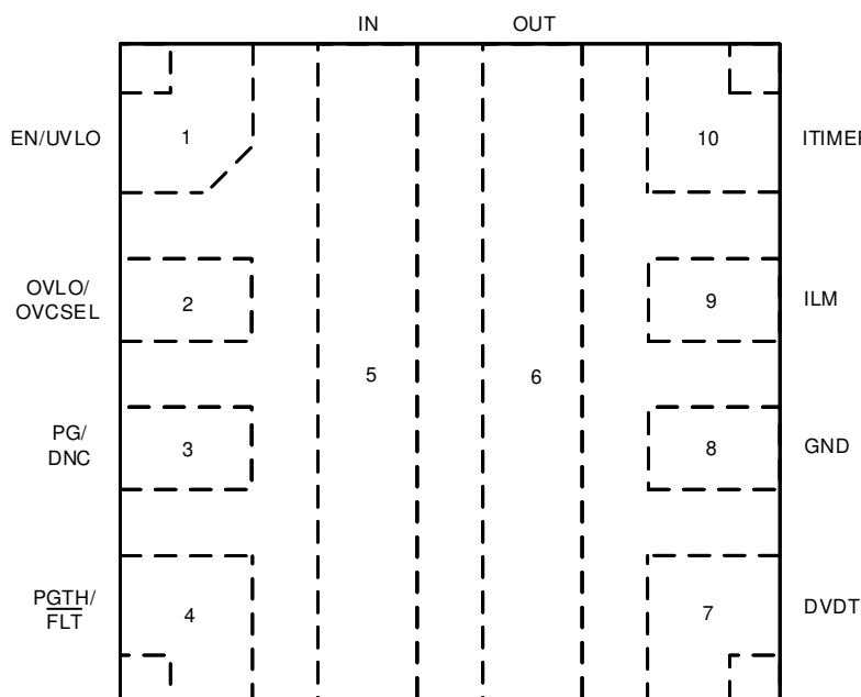
图 6-1. TPS2597xx RPW Package 10-Pin QFN (Top View)
