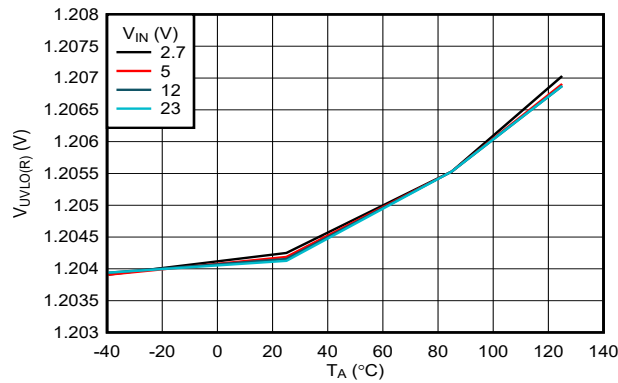
图 7-7. EN/UVLO Rising Threshold vs Temperature
