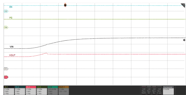
图 7-38. Overvoltage Clamp Response – TPS25972x
