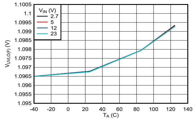
图 7-8. EN/UVLO Falling Threshold vs Temperature
