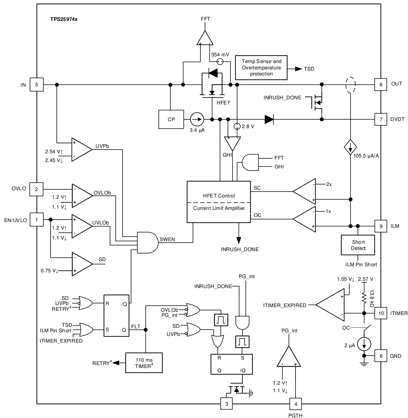
图 8-3. TPS25974x Block Diagram
