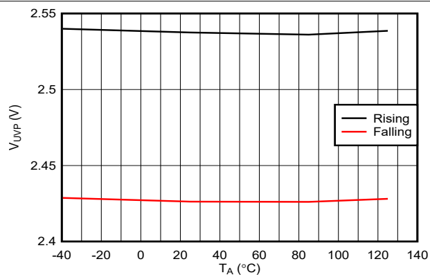
图 7-6. IN Undervoltage Threshold vs Temperature
