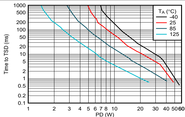
图 7-29. Time to Thermal Shut-Down During Steady State
