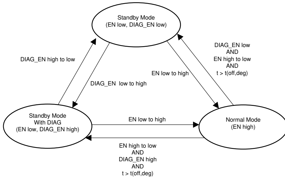
图 34. Working Modes
