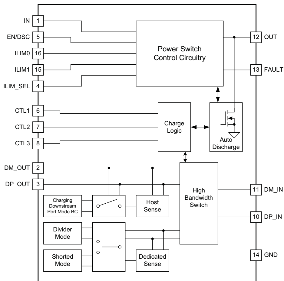
TPS2540/40A/41 Top-Level Functional Block Diagram
