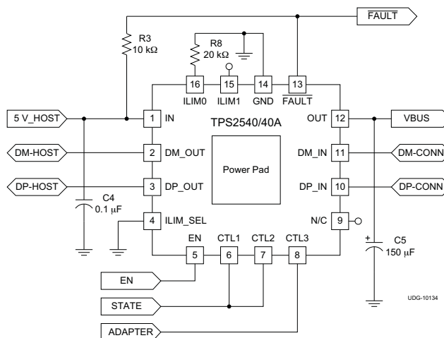
图 45. TPS2540/40A Application Using STATE and ADAPTER Control Signals
