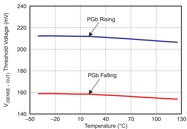
Figure 15. Threshold of V_{DS} vs Temperature, PGB Rising and Falling
