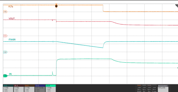
图 7-38. Overvoltage Clamp Response – TPS25972x
