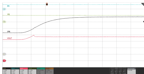
图 7-37. Overvoltage Clamp Response – TPS25972x
