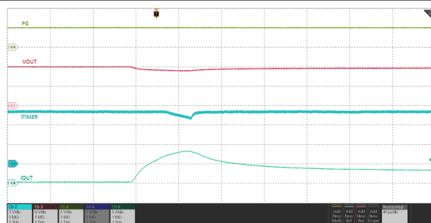
图 7-40. Active Current Limit Response – TPS25970x
