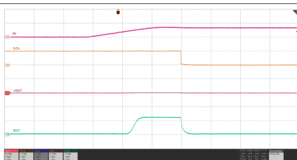
图 7-44. Output Short-Circuit During Steady State
