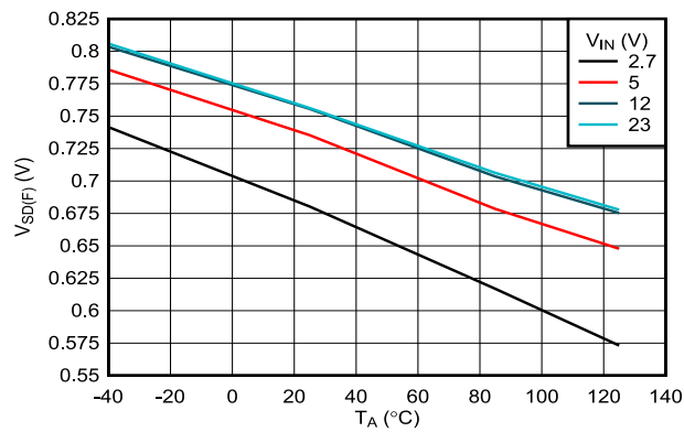
图 7-9. EN/UVLO Shutdown Falling Threshold vs Temperature
