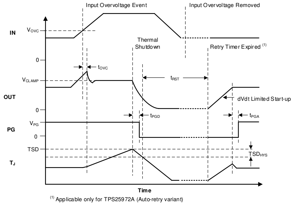
图 8-8. TPS25972x Overvoltage Response (Auto-Retry)
