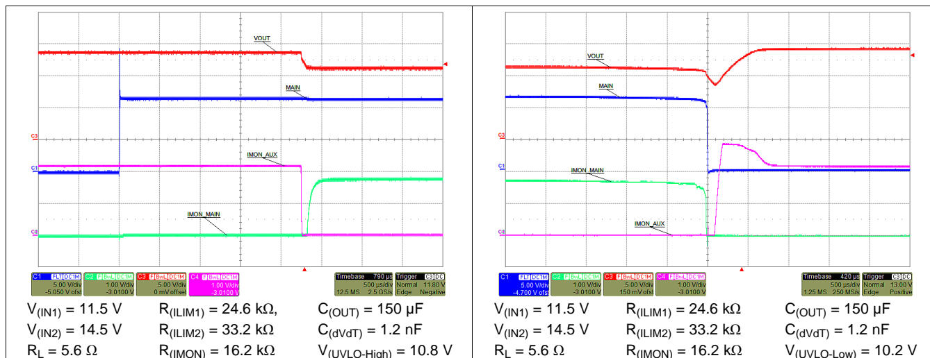
Figure 80. IN1 Power Recovery: Change Over from Auxiliary IN2 to Primary Power IN1
