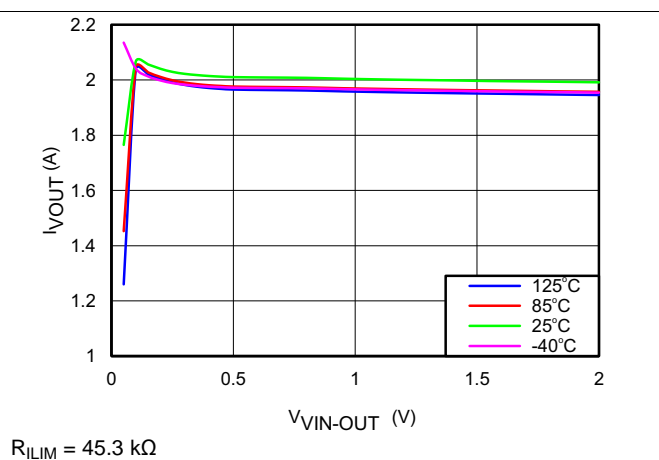
Figure 16. I_{VOU} vs V_{VIN-OUT}
