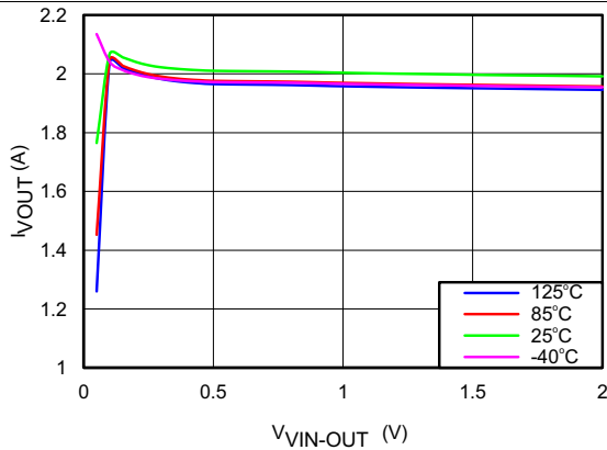
Figure 13. I_{VOUT} vs V_{VIN-OUT}
