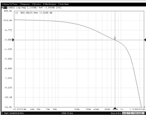
图 8-23. Data Transmission Characteristics vs Frequency
