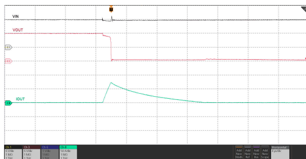
图 7-35. Circuit-Breaker Response
