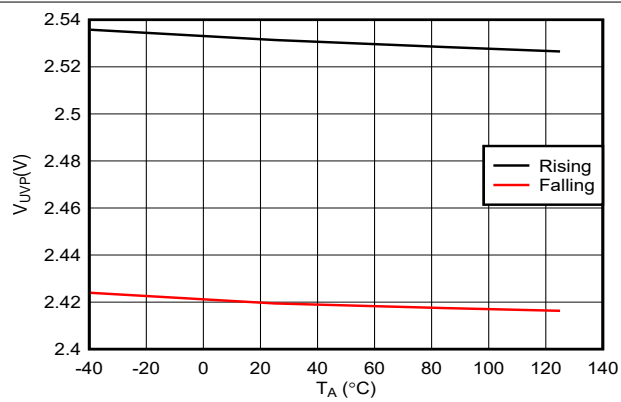
图 7-7. IN Undervoltage Threshold vs Temperature
