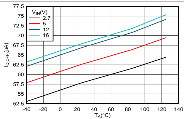
图 7-5. IN OFF State (UVLO) Current vs Temperature
