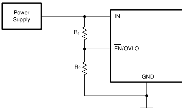
图 8-2. Adjustable Overvoltage Protection
