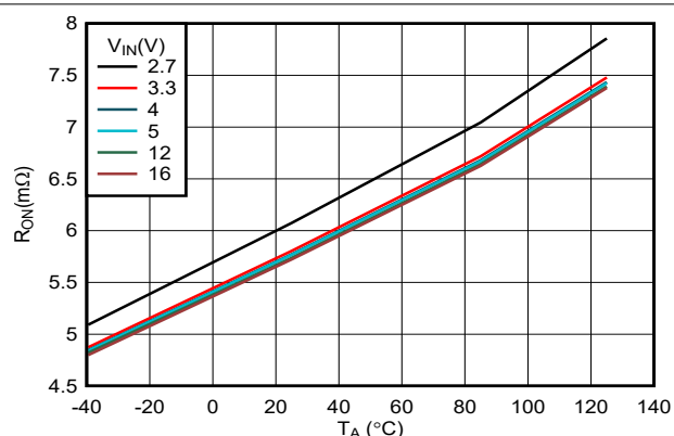
图 7-3. ON-Resistance vs Temperature ( I_{OUT} = 3\text{ A} )
