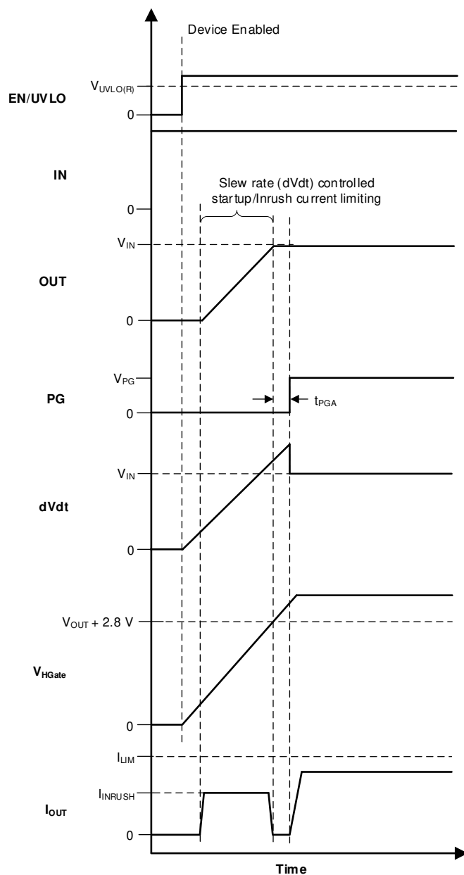
图 8-7. TPS25981xx PG Timing Diagram
