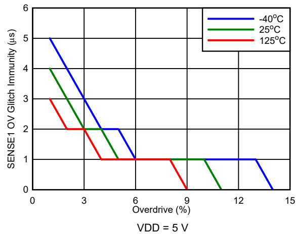
Figure 7-21. SENSE1 Glitch Immunity ( V_{\text{IT+}} ) vs Overdrive
