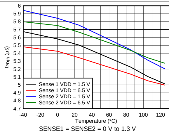
图 13. Propagation Delay from Sense High to Output High
