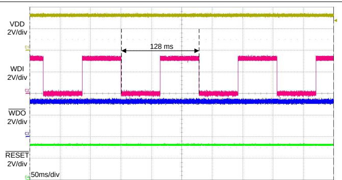
图 23. Typical WDI Signal
