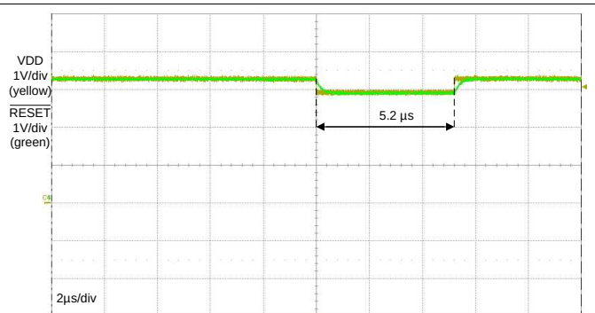
图 25. High to Low Glitch Immunity
