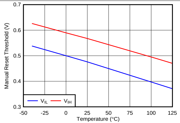
图 4. \overline{MR} Threshold vs Temperature
