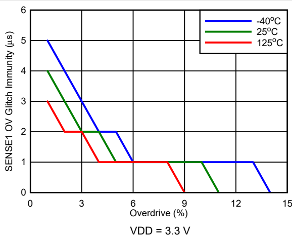
Figure 7-19. SENSE1 Glitch Immunity ( V_{IT+} ) vs Overdrive
