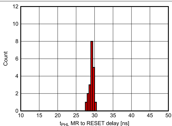
Figure 7-17. MR to RESET ( t_{PHL} ) Delay Histogram for TPS3705-33 Devices at 125°C (Unit Count = 20)
