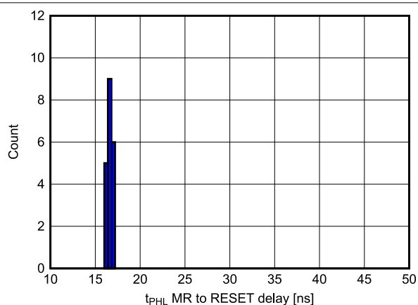
Figure 7-15. MR to RESET ( t_{PHL} ) Delay Histogram for TPS3705-33 Devices at -40°C (Unit Count = 20)
