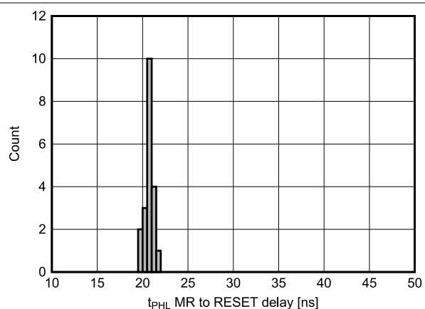
Figure 7-16. MR to RESET ( t_{PHL} ) Delay Histogram for TPS3705-33 Devices at 25°C (Unit Count = 20)
