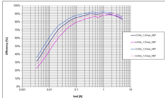
Figure 18. Efficiency
