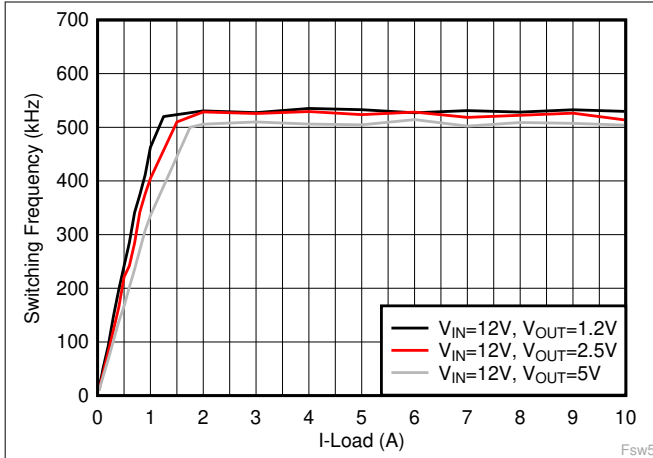
图 6-19. Switching Frequency vs Load Current, F_{sw} = 500 kHz, Eco-mode
