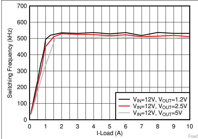
图 6-21. Switching Frequency vs Load Current, F_{sw} = 500 kHz, OOA
