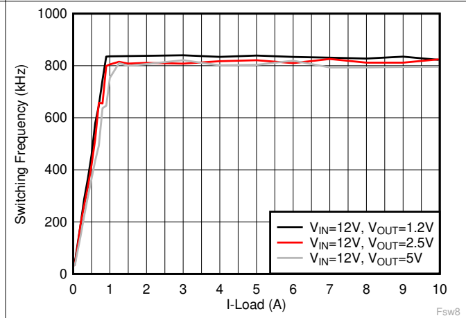
图 6-22. Switching Frequency vs Load Current, F_{sw} = 800 kHz, OOA
