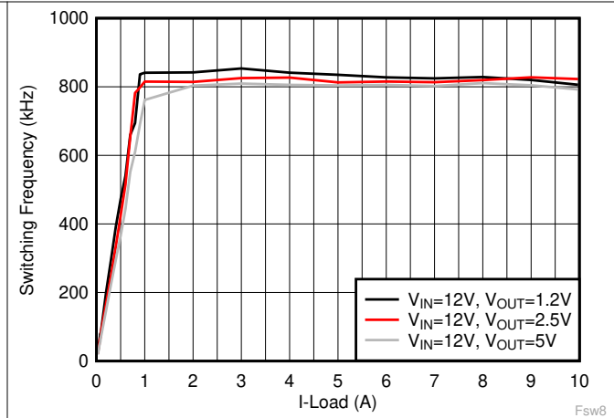
图 6-20. Switching Frequency vs Load Current, F_{sw} = 800 kHz, Eco-mode
