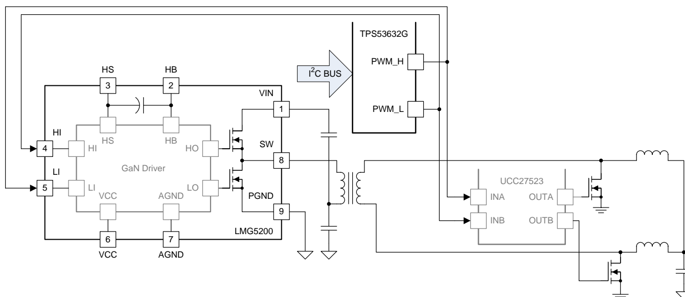
Simplified Schematic
