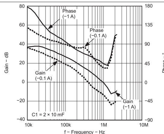
Figure 20. Bode Plot DDR2 Source
