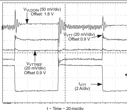
Figure 13. VTT Voltage Load Transient Response
