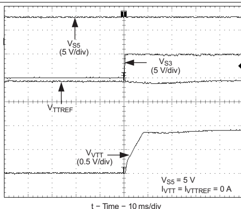
Figure 15. Startup Waveforms S3 Low-to-High
