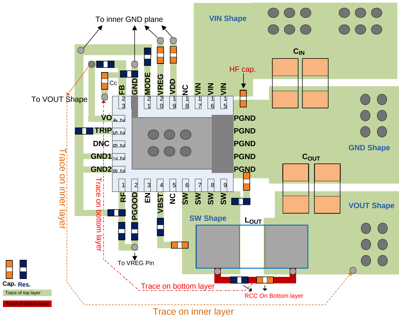
图 50. Layout Recommendation
