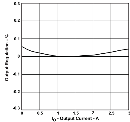
Figure 11. Output Regulation % vs. Output Current
