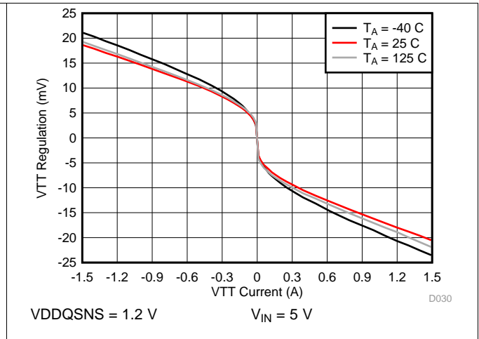
图 32. VTT Regulation to VTTREF vs I(VTT)
