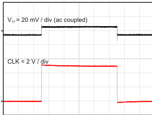
Time = 100 \mu sec / div 图 63. V_{TT} Output Transient Response
