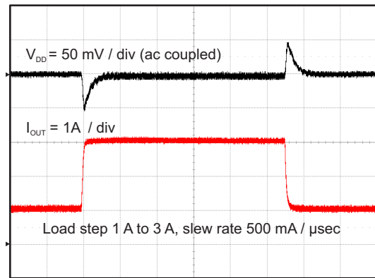
Time = 200 \mu sec / div 图 62. V_{DD} Output Transient Response
