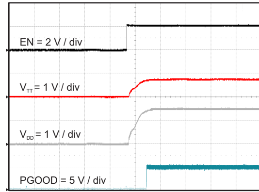
图 54. V_{TT} and V_{DD} Start-Up Relative to Enable
