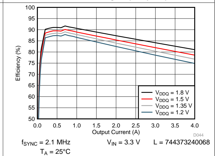
图 36. Efficiency
