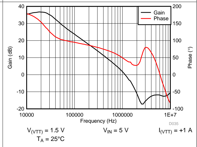
图 34. VTT Sourcing Frequency Response
