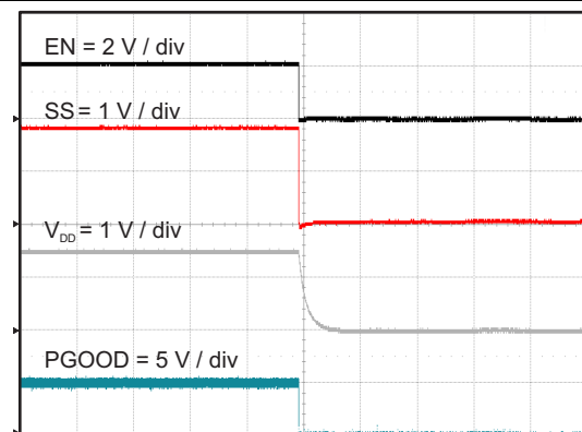
图 56. V_{DD} Shutdown Relative to Enable
