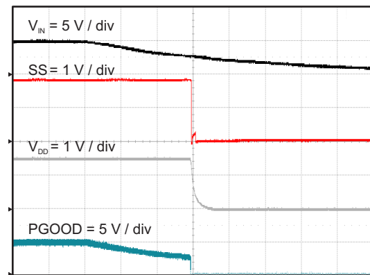
图 58. V_{DD} Shutdown Relative to V_{IN}
