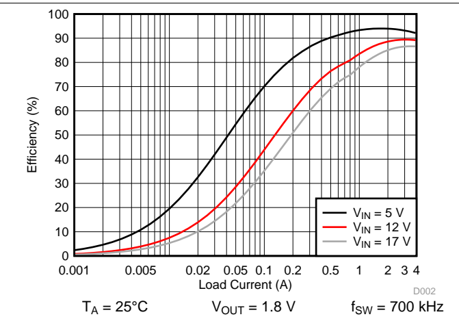
图 37. Efficiency (Log Scale)
