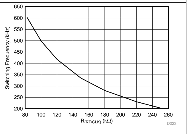
图 24. Switching Frequency vs RT/CLK Resistor (Low Range)
