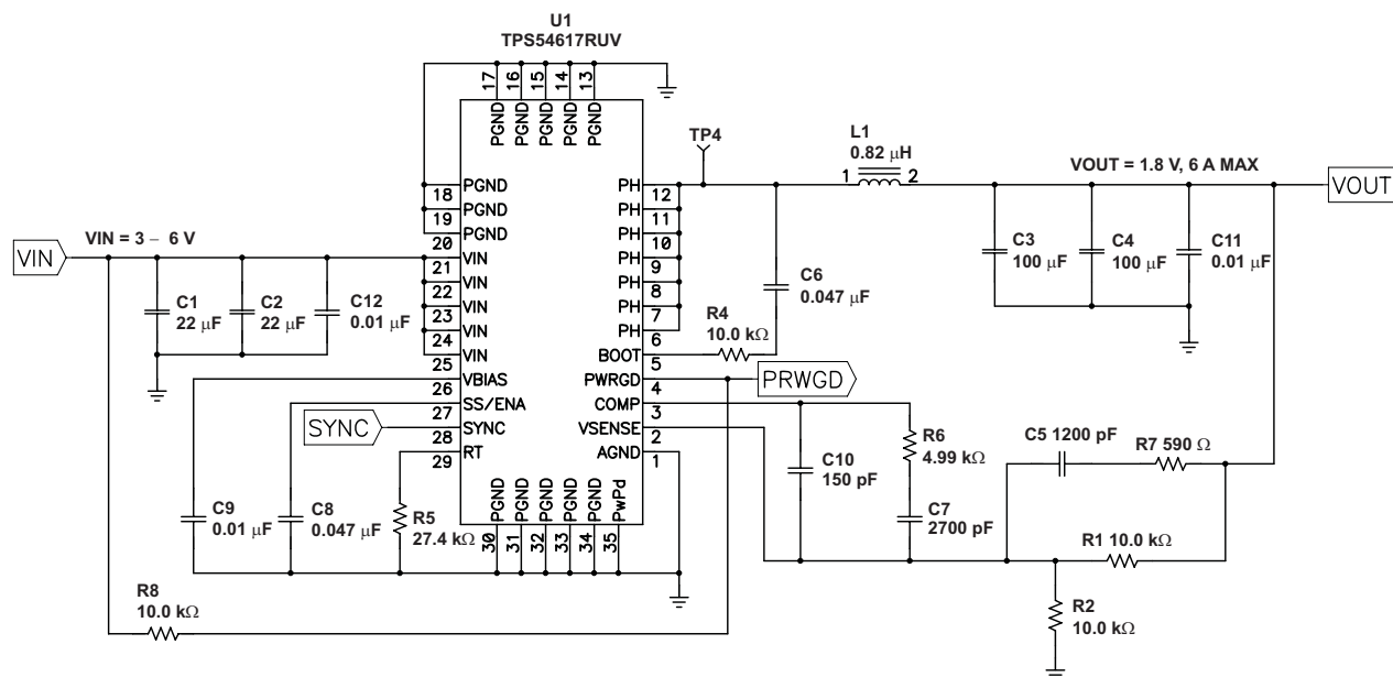
Figure 10. Application Circuit
