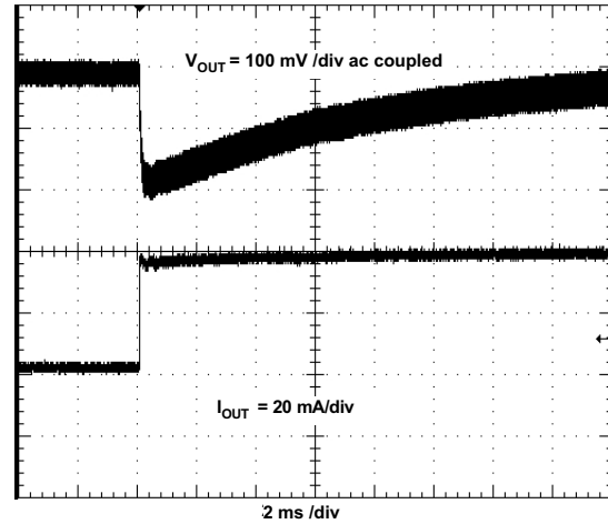
Figure 46. Load Transient
