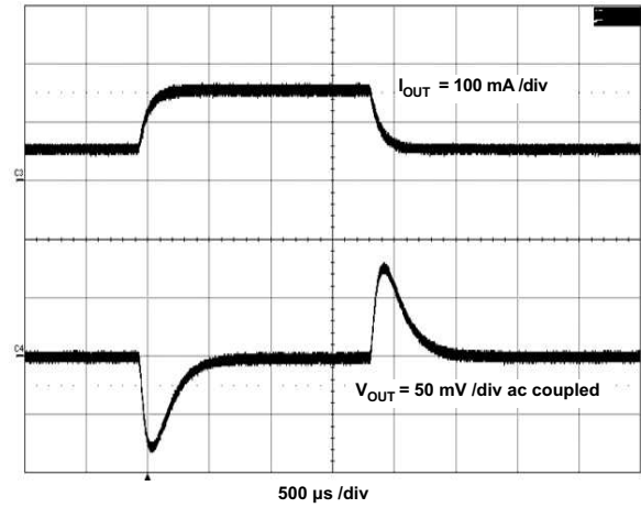
Figure 28. Load Transient
