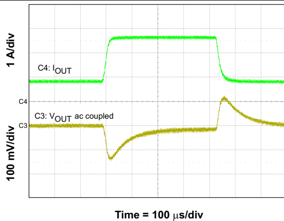
Figure 34. Load Transient
