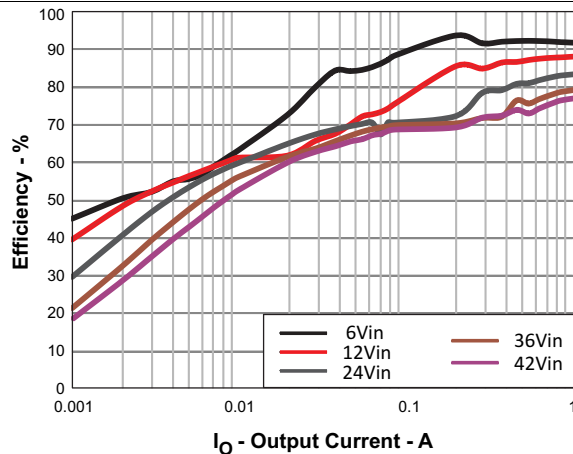
Figure 45. Light-Load Efficiency
