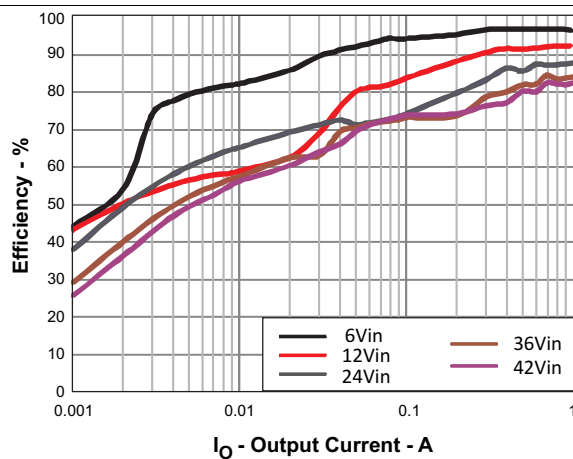
Figure 47. Light-Load Efficiency
