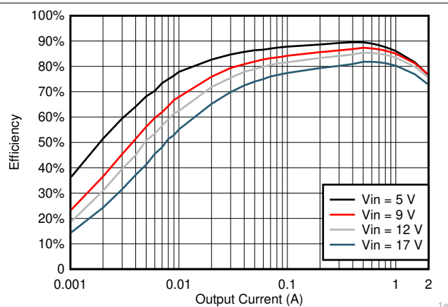
图 7-10. V_{OUT} = 1.05V 效率, L = 2.2\mu H
