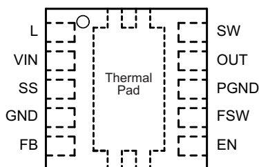
Pin Functions
