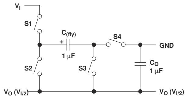
图 9-12. Step-Down Principle
