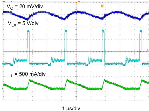
图 8-8. TPS562201 Output Voltage Ripple, I_{OUT} = 0.25 \text{ A}
