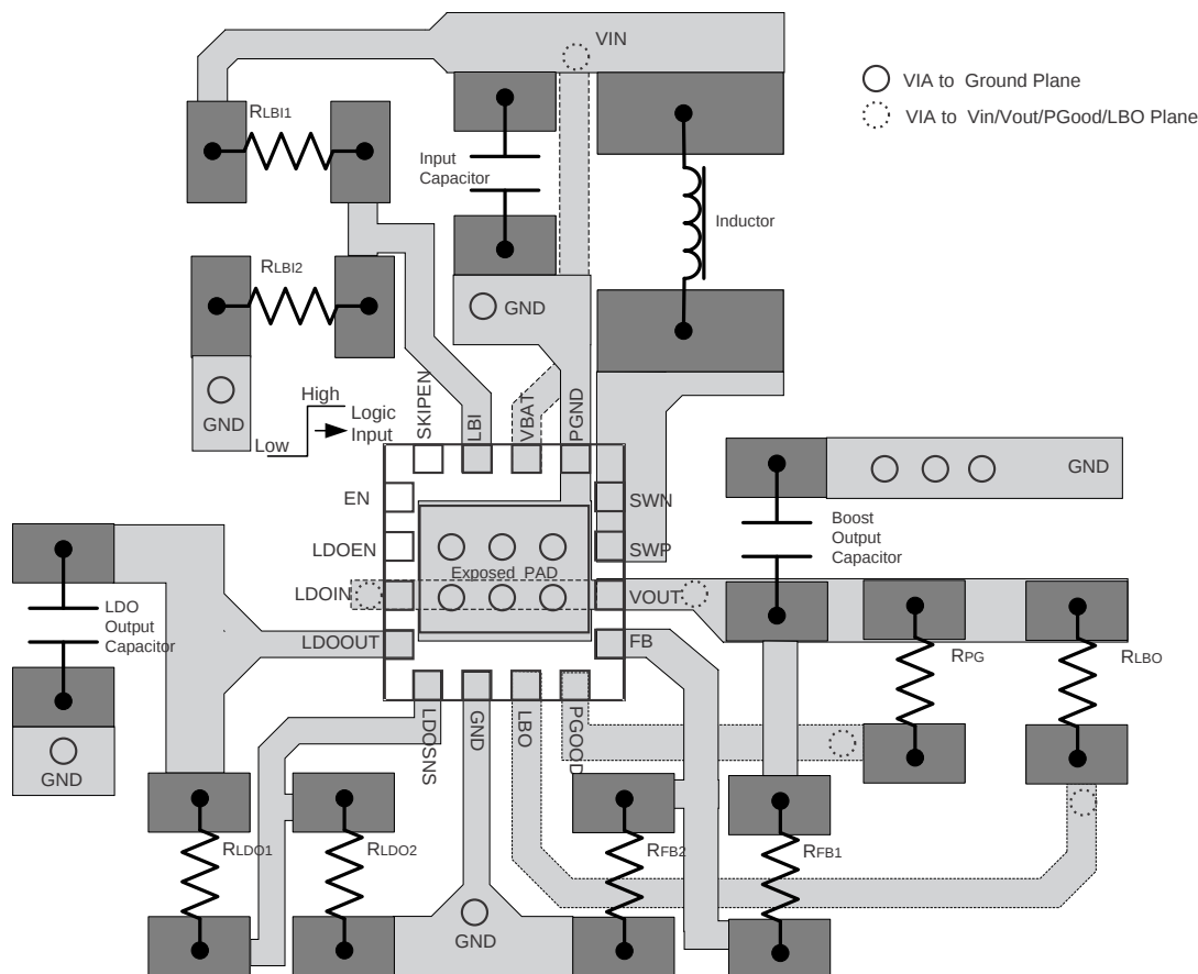
Figure 32. Layout Example
