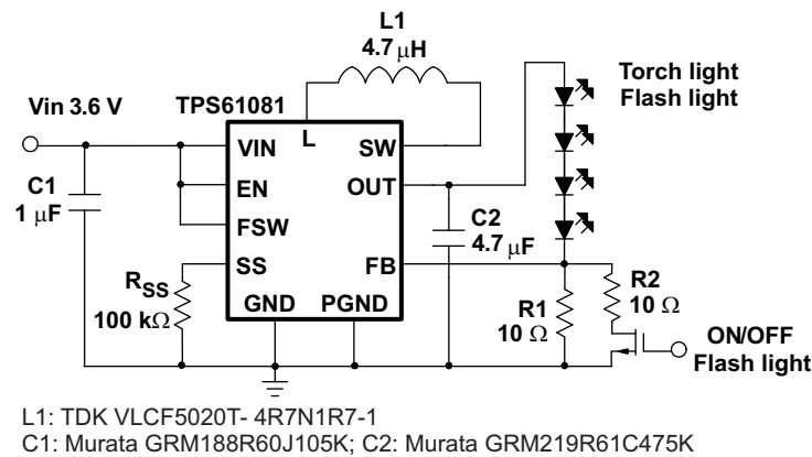
Figure 21. 50 mA Torch Light and 100 mA Flash Light
