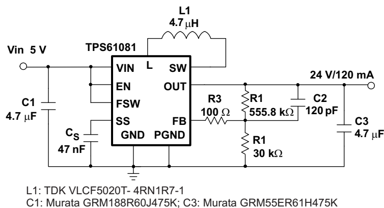
Figure 22. 5 V to 24 V, 120 mA Step-Up DC-DC Converter
