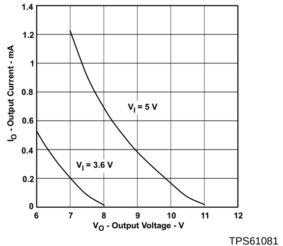
Figure 20. Minimum Load Requirement
