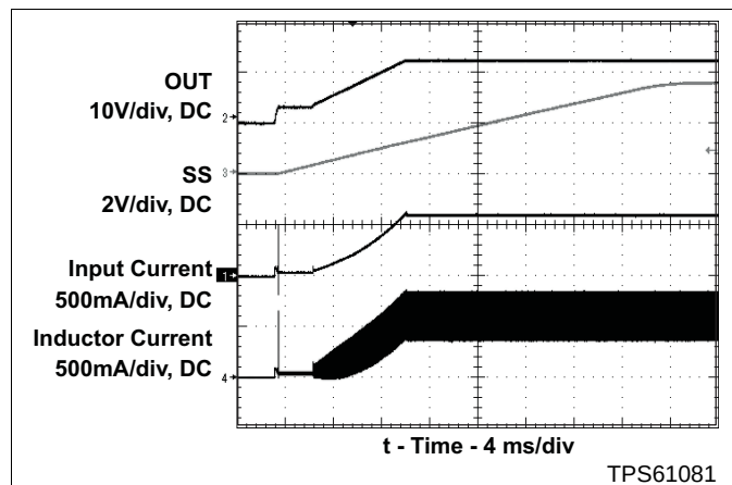
Figure 13. Soft Start
