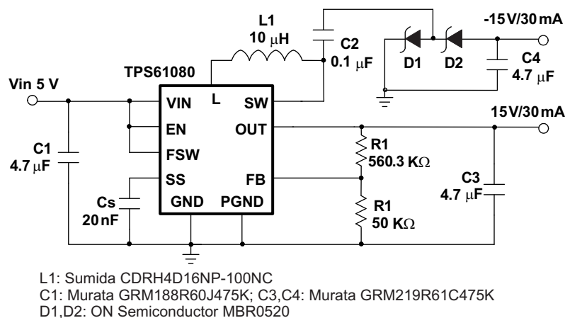
Figure 24. \pm 15 V Dual Output Converter
