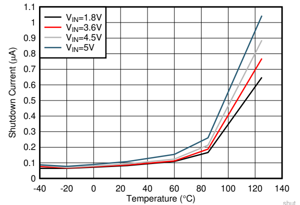
图 6-8. Shutdown Current vs Temperature
