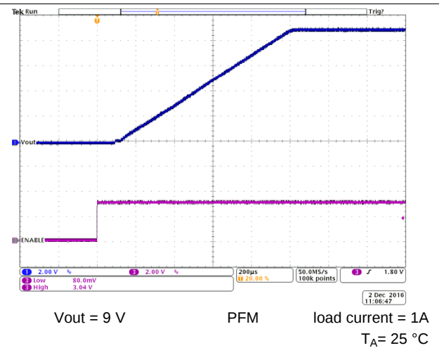
Figure 63. Start-Up Timing
