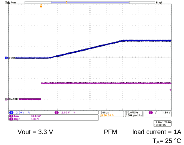
Figure 49. Start-Up Timing
