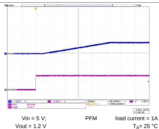
Figure 35. Start-Up Timing
