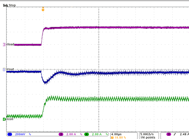
图 9-30. PWM-PSM-Transition
