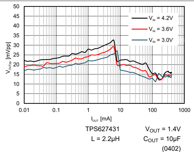
图 9-13. Typical Output Ripple Voltage V_{OUT} = 1.4\text{ V}
