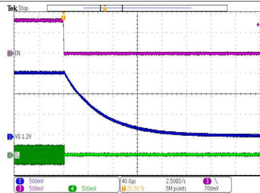
TPS62801 V_{OUT} = 1.2\text{ V} VSEL/MODE = V_{IN} \text{EN} = \text{high to low} No Load
