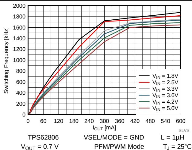
图 34. Switching Frequency vs. Output Current
