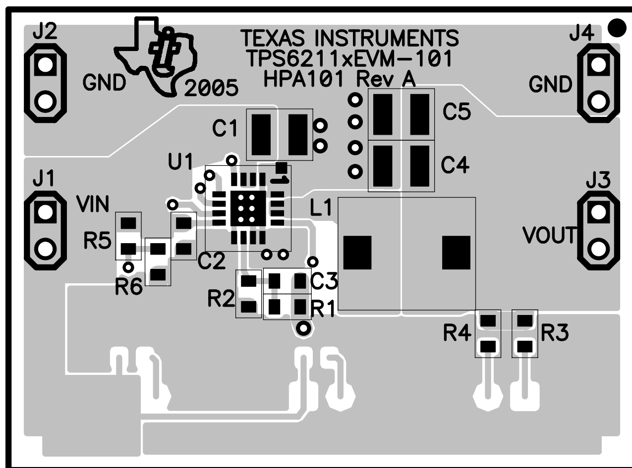
Figure 22. Recommended Layout
