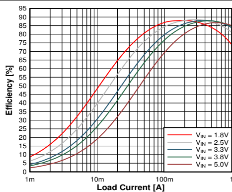
V_{OUT} = 1.1\text{ V} Forced PWM Operation
