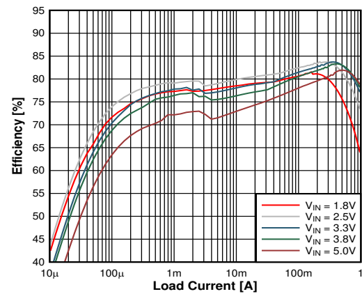
V_{OUT} = 0.6\text{ V} Auto Power Save Mode
