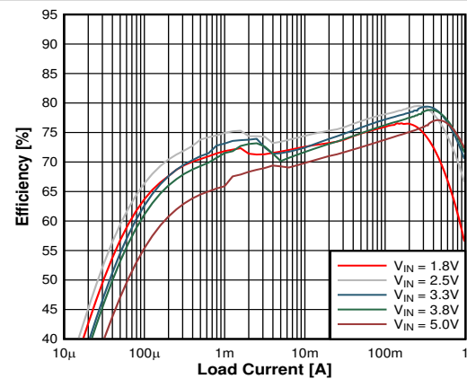
V_{OUT} = 0.4\text{ V} Auto Power Save Mode
