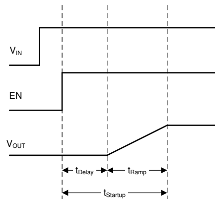
图 8-2. Start-up Sequence
