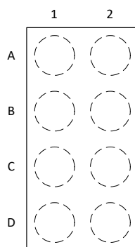
图 6-1. 8-Pin DSBGA YCH Package (Top View)
