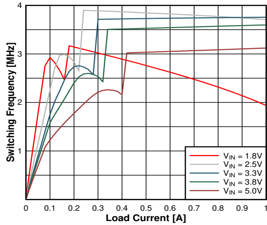
图 9-8. Switching Frequency
