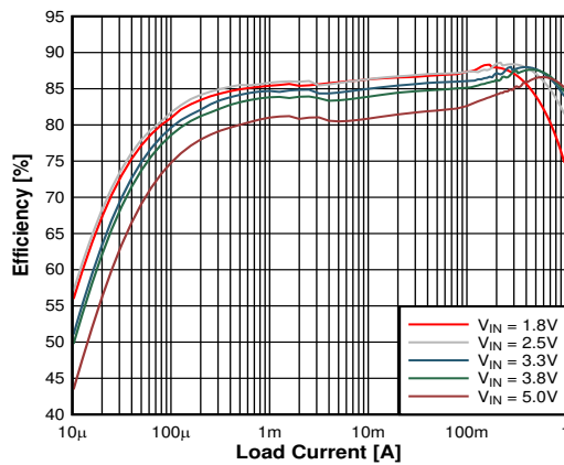
V_{OUT} = 1.1\text{ V} Auto Power Save Mode
