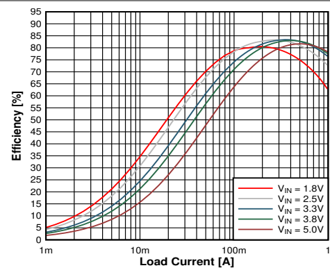
V_{OUT} = 0.6\text{ V} Forced PWM operation
