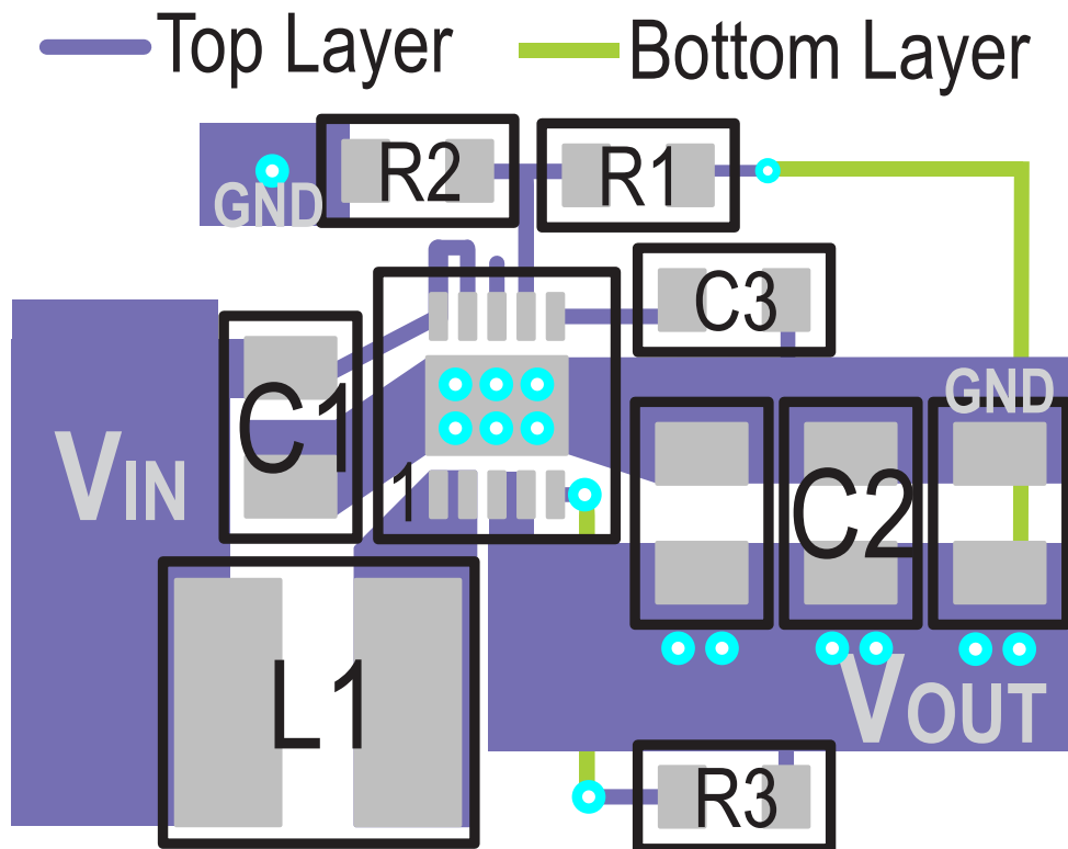
图 37. Layout Recommendation
