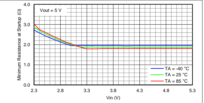
图 14. Minimum Resistance at Startup
