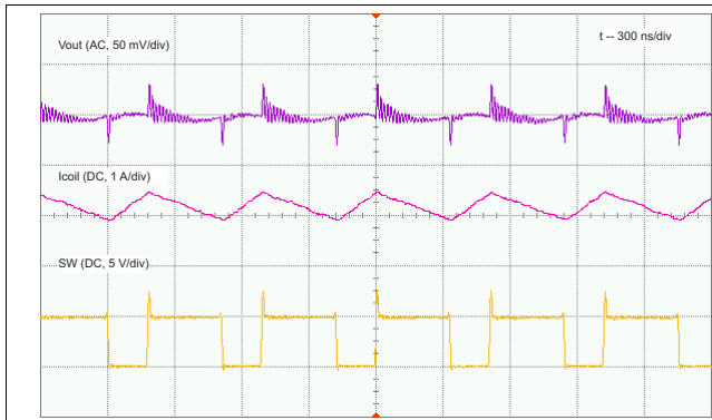
图 19. PWM Operation ( V_{OUT} = 5\text{ V} , I_{OUT} = 2\text{ A} )
