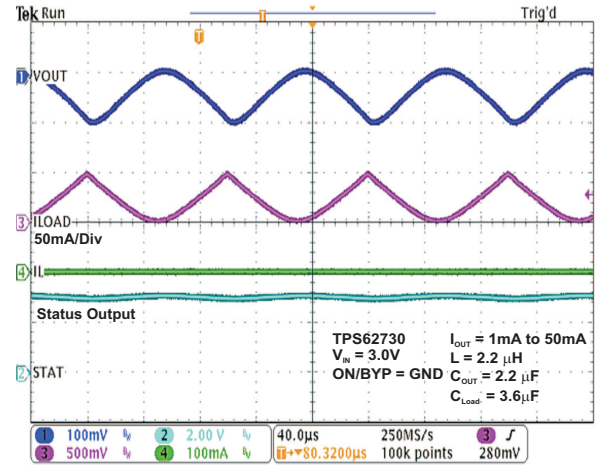
Figure 26. Bypass Mode Operation V_{OUT} AC Behavior ON/BYP = \text{GND}
