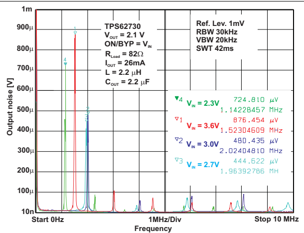
Figure 28. Spurious Output Noise TPS62730 I_{OUT} 26\text{ mA}
