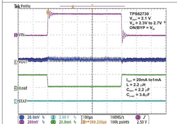
Figure 23. DC-DC Mode Operation Line and Load Transient Performance
