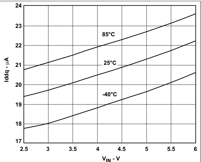
Figure 2. I_q For One Converter, Not Switching
