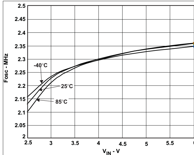
Figure 1. F_{OSC} vs V_{IN}
