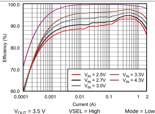
图 51. TPS61282A Efficiency vs Output Current
