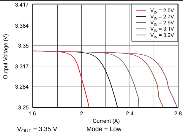
图 36. TPS61281A DC Output Voltage vs Output Current
