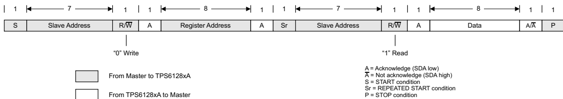
图 25. “Read” Data Transfer Format in Standard-, Fast, Fast-Plus Modes
