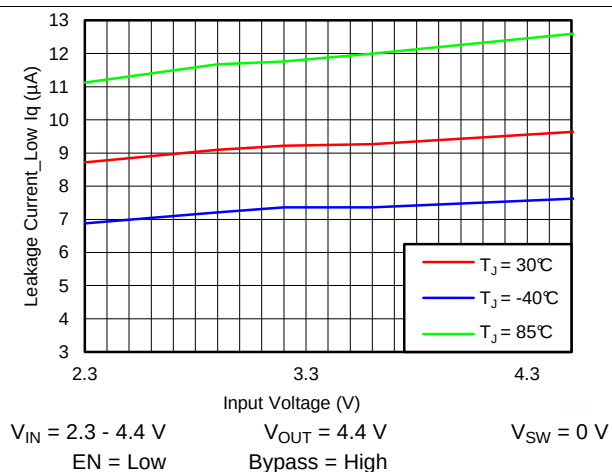
图 10. Shutdown Current vs Input Voltage
