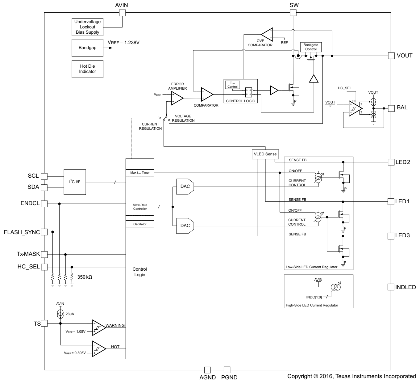
Figure 33. TPS61306 Block Diagram
