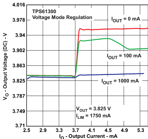
Figure 18. DC Output Voltage vs Load Current
