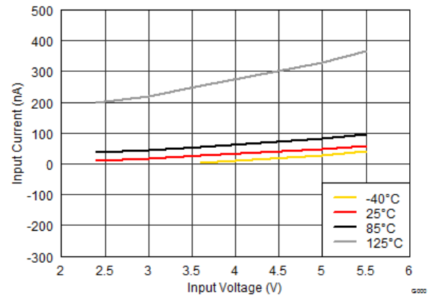
图 2. Shutdown Current
