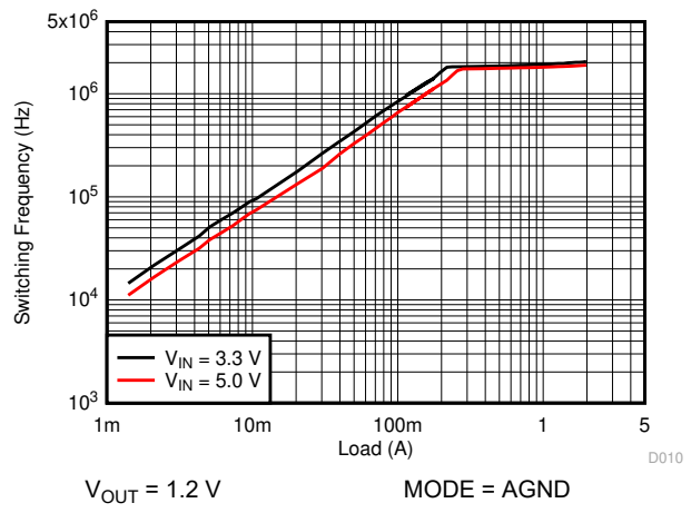
图 9-11. Switching Frequency, PWM/PSM Mode (2.0 MHz)
