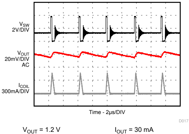
图 9-16. Output Ripple, Power Save Operation
