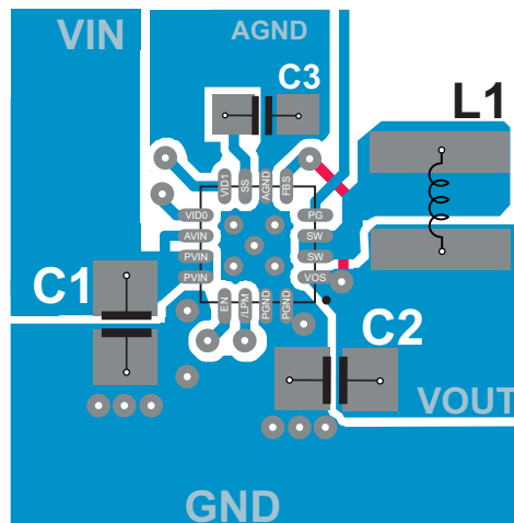
图 18. TPS62134x Layout Example
