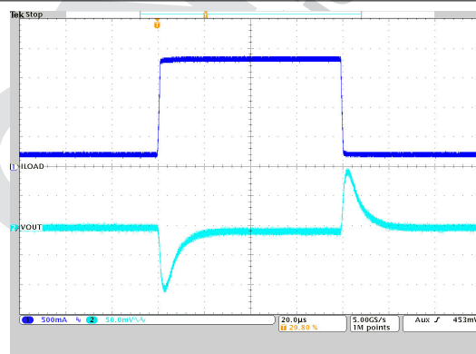
图 10-27. Load Transient Response
