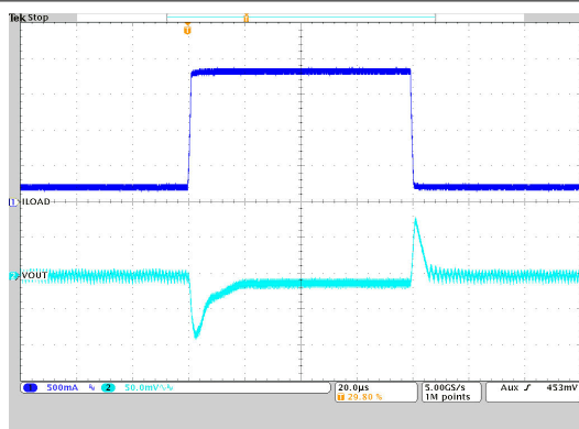
图 10-26. Load Transient Response
