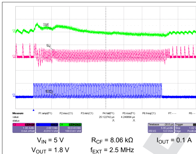
图 10-59. Switching from External Synchronization to Power-Save Mode (PFM)
