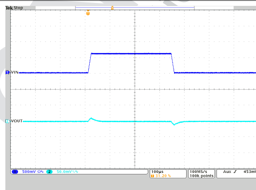
图 10-39. Line Transient Response
