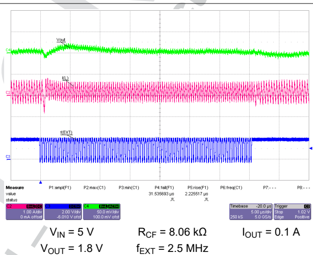
图 10-60. Switching from External Synchronization to Internal Fixed Frequency
