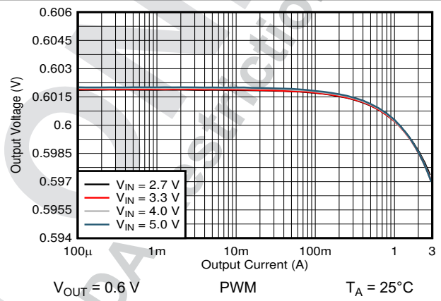
图 10-17. Output Voltage versus Output Current
