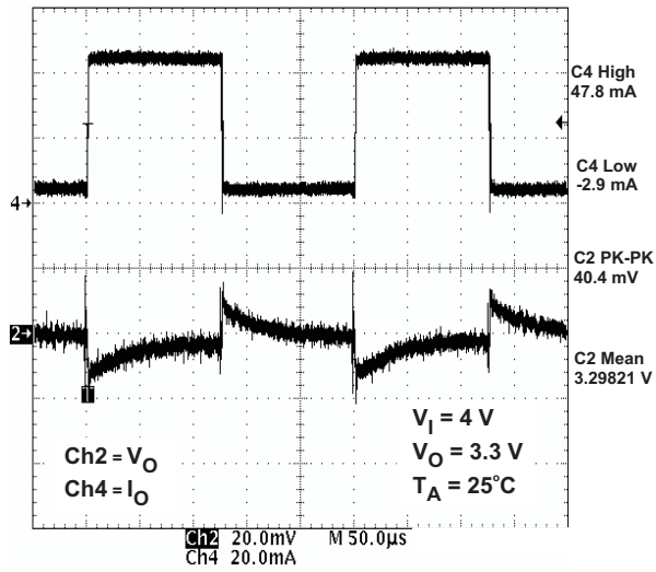
Figure 27. LDO2 Load Transient Response
