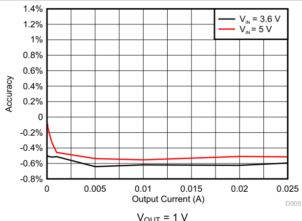
图 7-5. DCDC5 Accuracy
